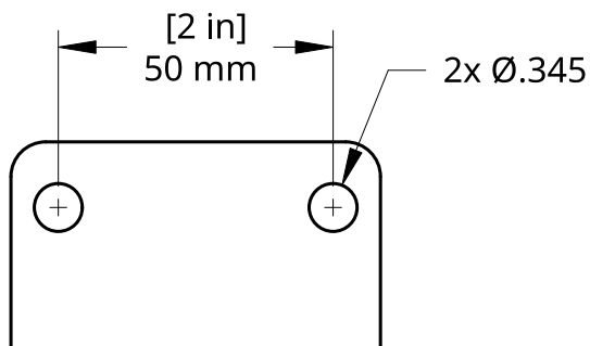
MOUNTING HOLE PATTERN (Do Not Scale)
