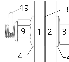
10*ASSEMBLED SIDE VIEW
